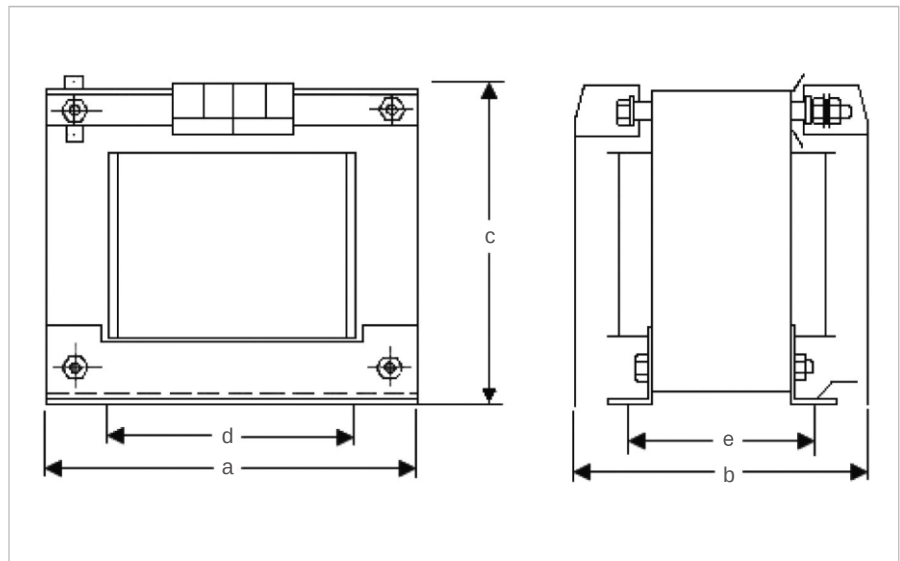
ST Transformer
