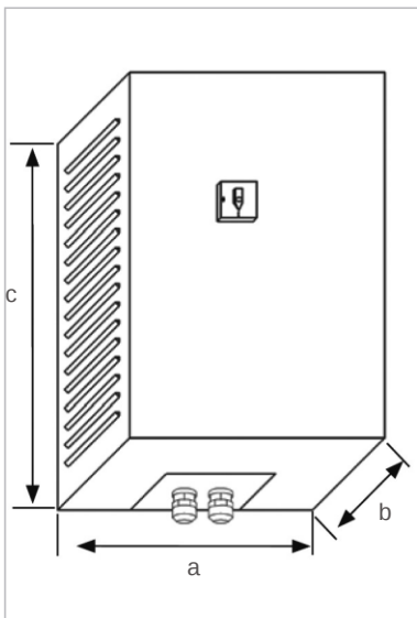
SLSH Transformer
